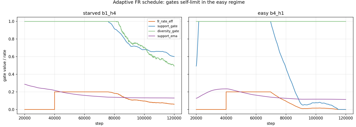
Figure 25: Adaptive FR schedule trajectories for a starved and an easy cell. The effective rate stays near its base value while the (exogenous, marginal-flatness) support gate is high in the starved cell, and is throttled by the support gate and warm-up in the already-accurate cell, with the diversity gate providing the genealogy safeguard.
