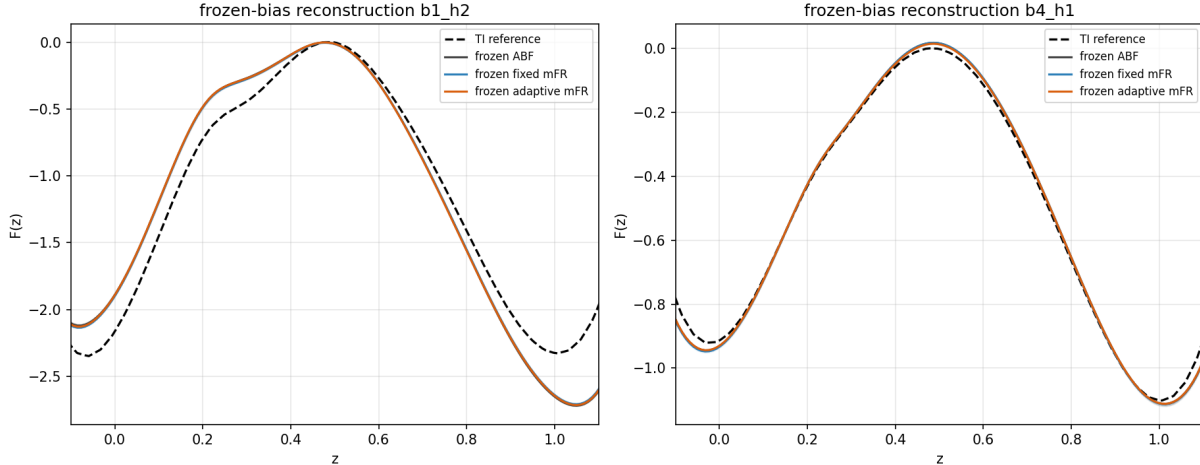
Figure 27: Frozen-bias reconstruction (27) from the learned ABF, fixed-mFR and adaptive-mFR biases (median and IQR over independent frozen seeds) against the TI reference, for a starved and an easy cell.
