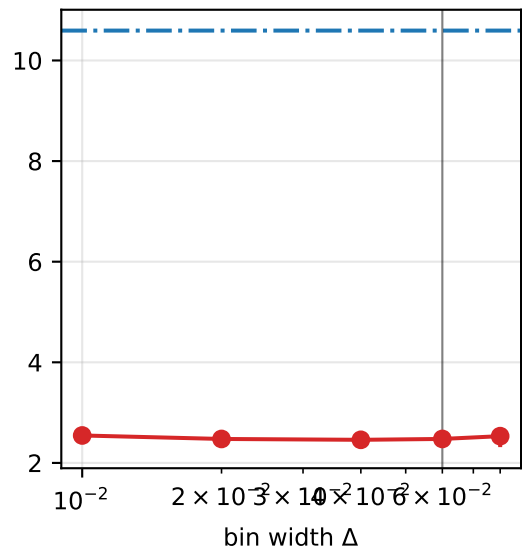
Entropic bottleneck, ABF-only bin-width calibration (8 seeds); selected Delta = 0.060
