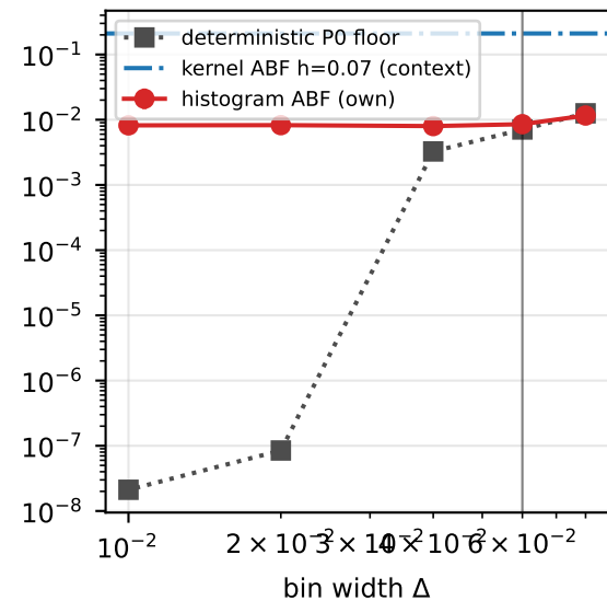
Entropic bottleneck, ABF-only bin-width calibration (8 seeds); selected Delta = 0.060
