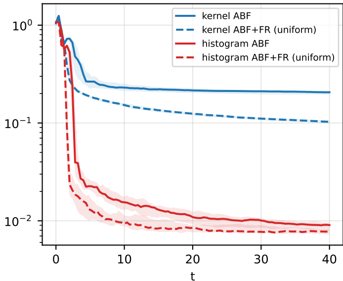
Entropic bottleneck confirmation (20 seeds; kernel h=0.07 vs histogram \Delta=0.060 ); median + IQR e_F(t) e_{F'}(t) (own estimator)
