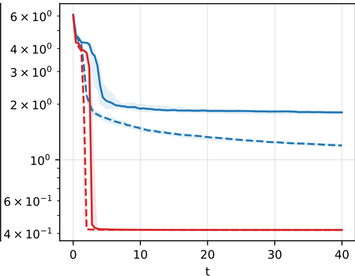
Entropic bottleneck confirmation (20 seeds; kernel h=0.07 vs histogram \Delta=0.060 ); median + IQR e_F(t) e_{F'}(t) (own estimator)
