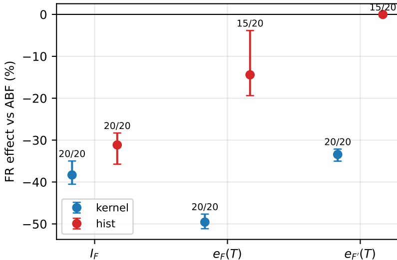
Entropic bottleneck: FR effect by estimator
