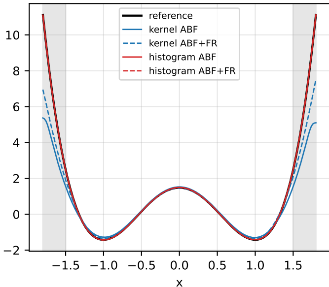
final F (seed-median profile)
