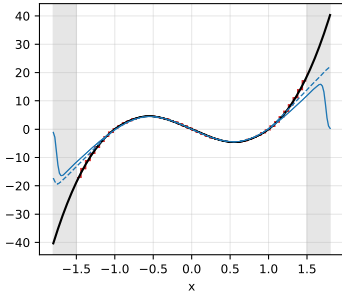
final F' (kernel: grid; histogram: bins)
