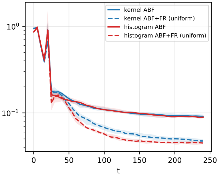
WCA dimer confirmation (16 seeds); kernel at h_{\text{read}}^*=0.0125 , histogram n_{\text{bins}}=160 (own); median + IQR
