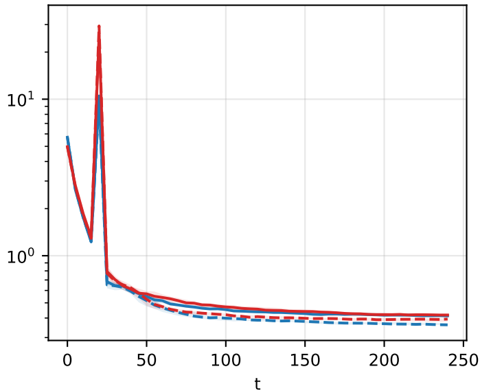
WCA dimer confirmation (16 seeds); kernel at h_{\text{read}}^*=0.0125 , histogram n_{\text{bins}}=160 (own); median + IQR
