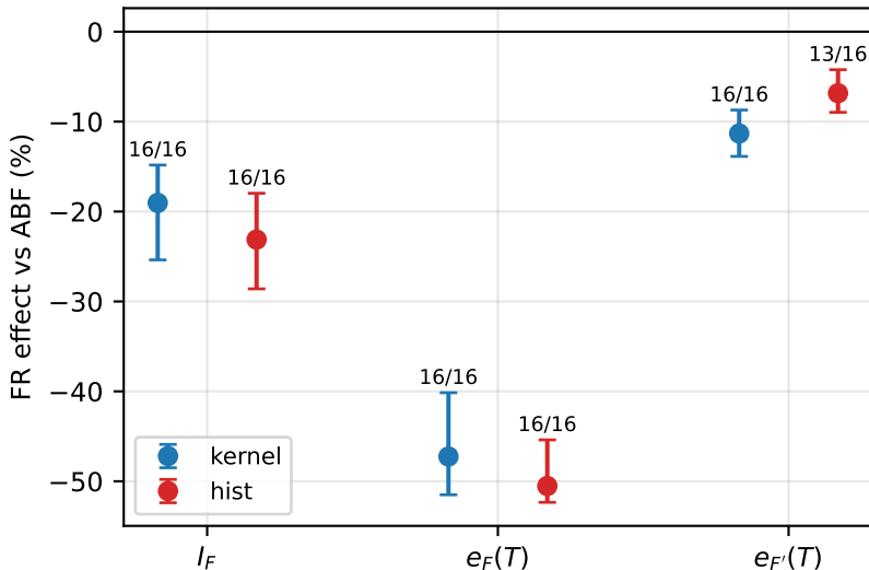
WCA dimer: FR effect by estimator
