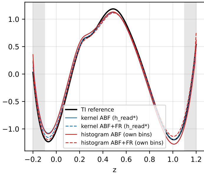
final F (seed-median profile)
