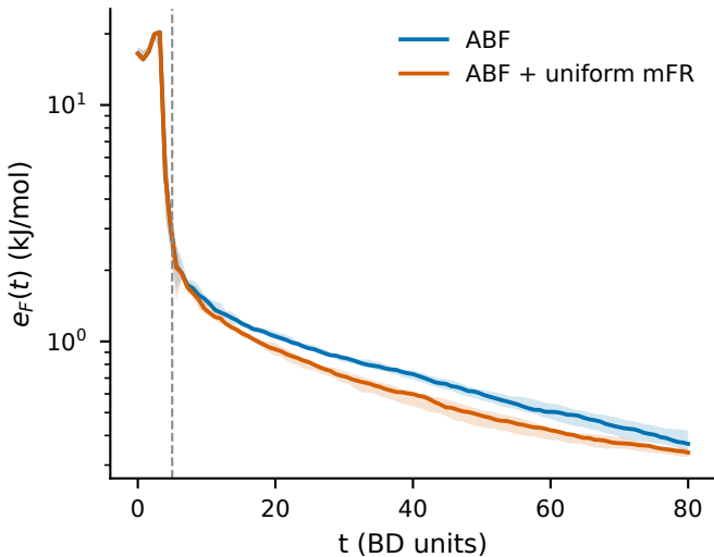
ethene 450 K
