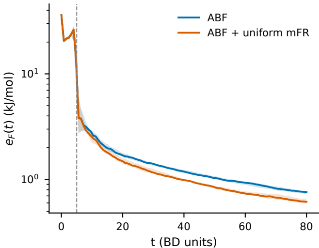
propene 450 K
