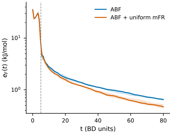
propene 600 K
