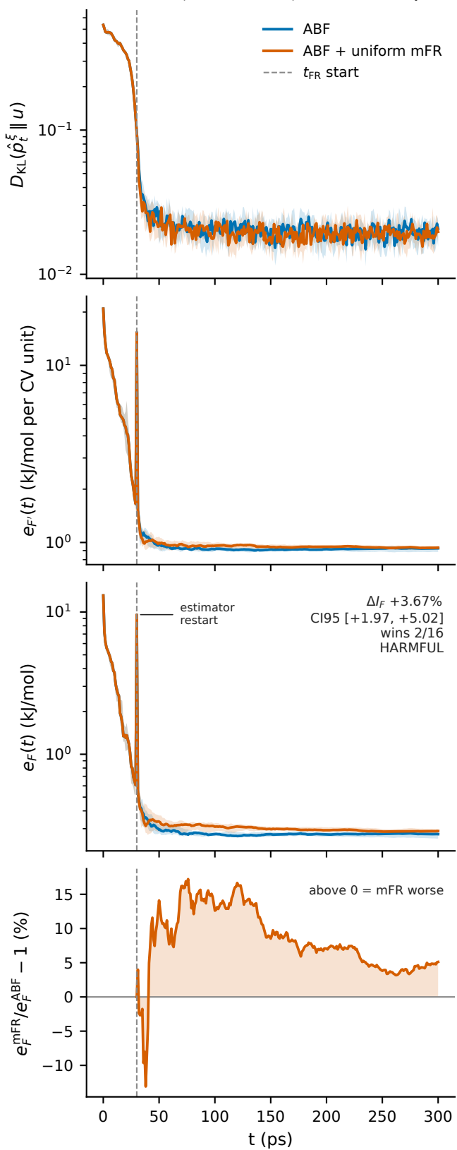
Ethane/ZIF-8 300 K 16 seeds, FR rate 0.05; median and IQR
