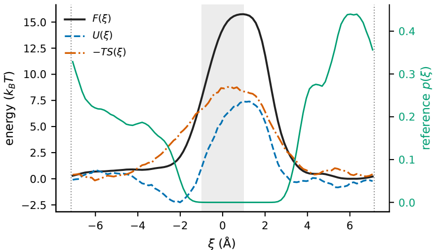
Ethane/ZIF-8 300 K umbrella reference (shaded: |\xi| < \delta_w ; dotted: cages \xi_A, \xi_B )
