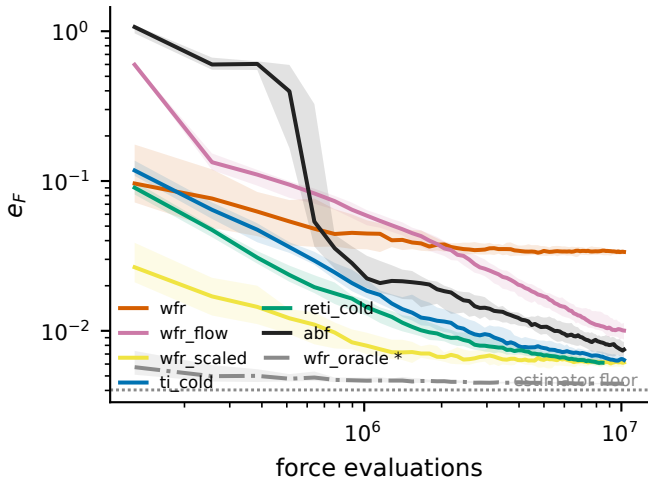
EB: convergence at matched cost
