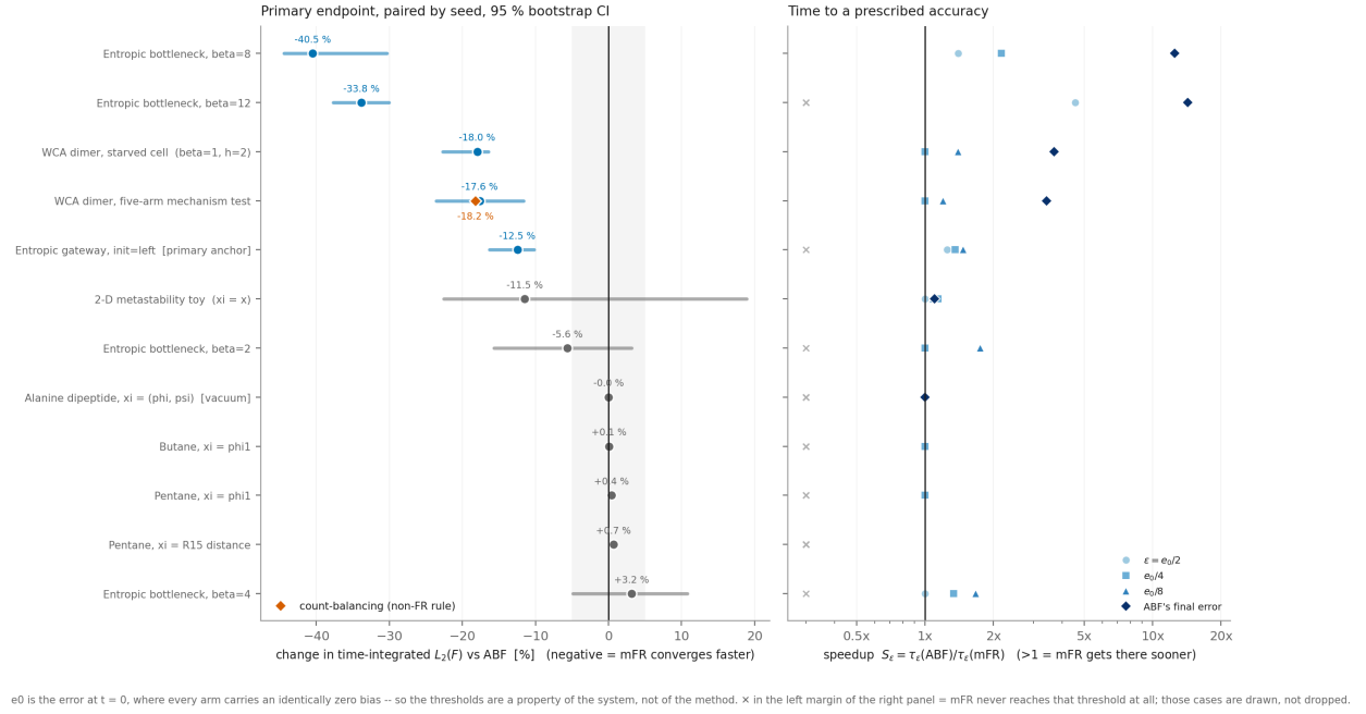
Figure 50: Left: the preregistered endpoint with its bootstrap interval, the shaded band the \pm 5\% practical-equivalence margin. The single orange marker is count balancing (Section 20.5), plotted on the one cell where it exists because omitting it would make the summary read as stronger evidence for Fisher–Rao than the data support. Right: S_\epsilon of Equation (44) at the four declared thresholds, on a logarithmic axis; the threshold family is ordered, so it is drawn as a sequential ramp rather than as four unrelated colours. Crosses at the left edge are censored cells.
