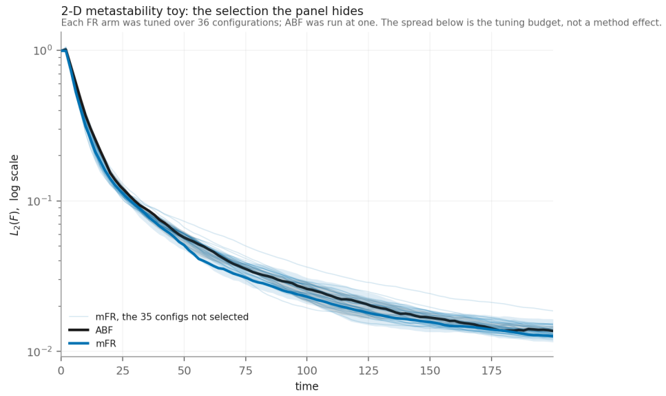
Figure 52: The tuning asymmetry in the metastability model. Faint lines are the 36 - 1 estimated-target configurations that were not selected; the heavy blue line is the one that was, and the black line is the single ABF configuration it is compared against. The spread is the tuning budget, not a method effect.
