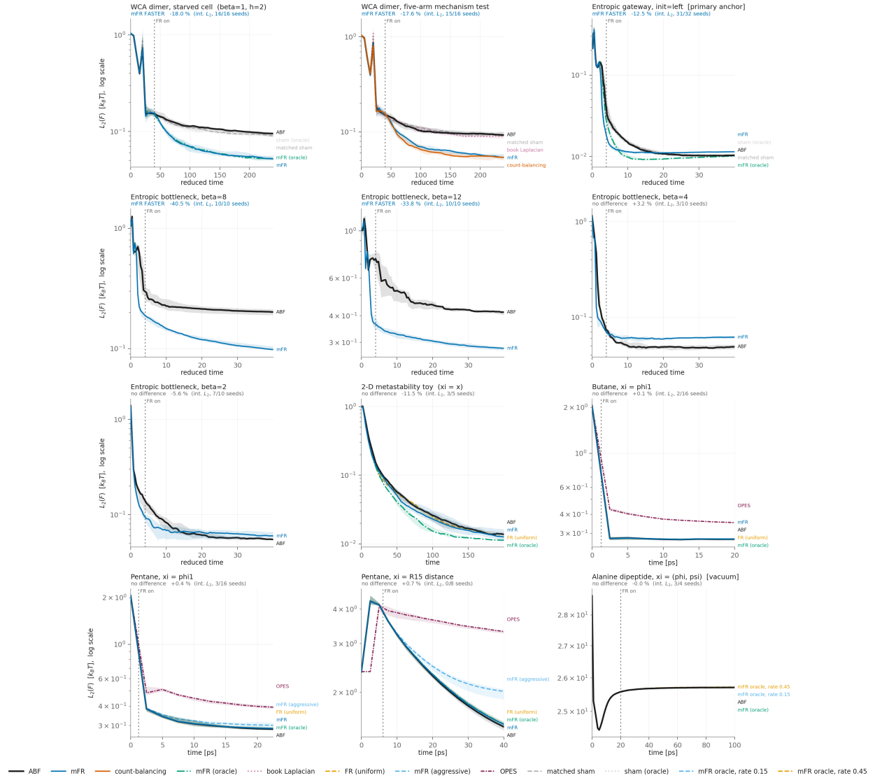
Figure 49: The convergence atlas: e_F(t) of Equation (43) for every benchmark in this report that has both an ABF and an mFR arm. Median over seeds, band the inter-quartile range, logarithmic ordinate. The dotted vertical rule marks the step at which the birth–death mechanism is enabled; before it the arms differ only by seed noise, which is the visual null control every panel carries for free. The header of each panel states the regime assigned by the preregistered endpoint and its own confidence interval, never by eye. Systems with no mFR arm — methane, sodium chloride, valine, deca-alanine, C60 — cannot appear and are not drawn; their absence is a protocol outcome, recorded in results/convergence_atlas/atlas.json , not an omission.
