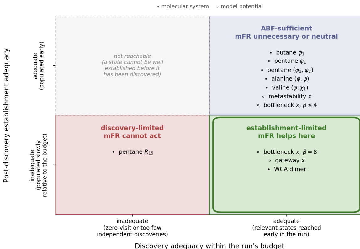
Figure 53: The regime map, on categorical axes. Both axes are two-state because that is what the evidence supports: each system carries a discovery verdict and an establishment verdict, not a continuous adequacy score, and interpolating coordinates to draw a scatter plot would present a classification as a measurement. The upper-left cell is empty by construction — a state cannot be well established before it has been discovered. Only the outlined cell is mFR's. Generated from results/closure/v1_regime_map.csv by report/scripts/make_regime_map_figure.py .
