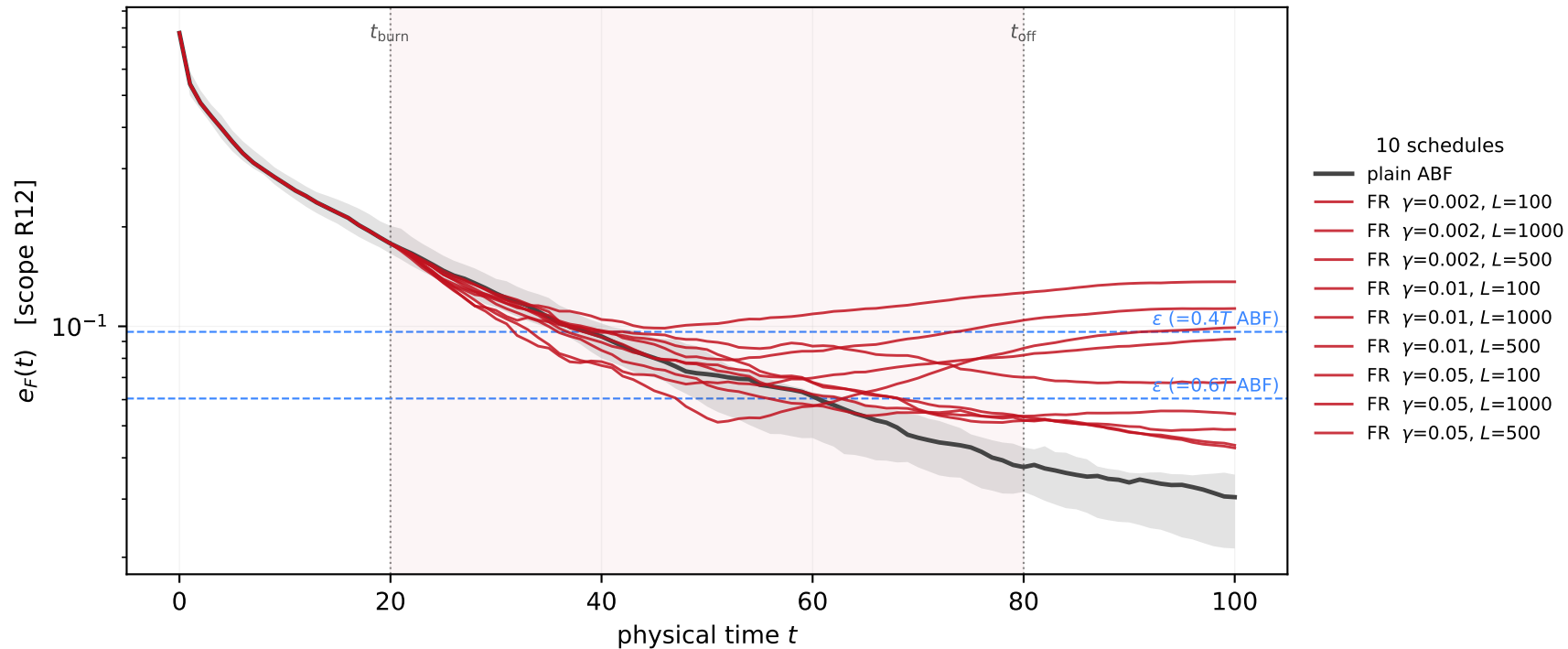
Free-energy convergence
