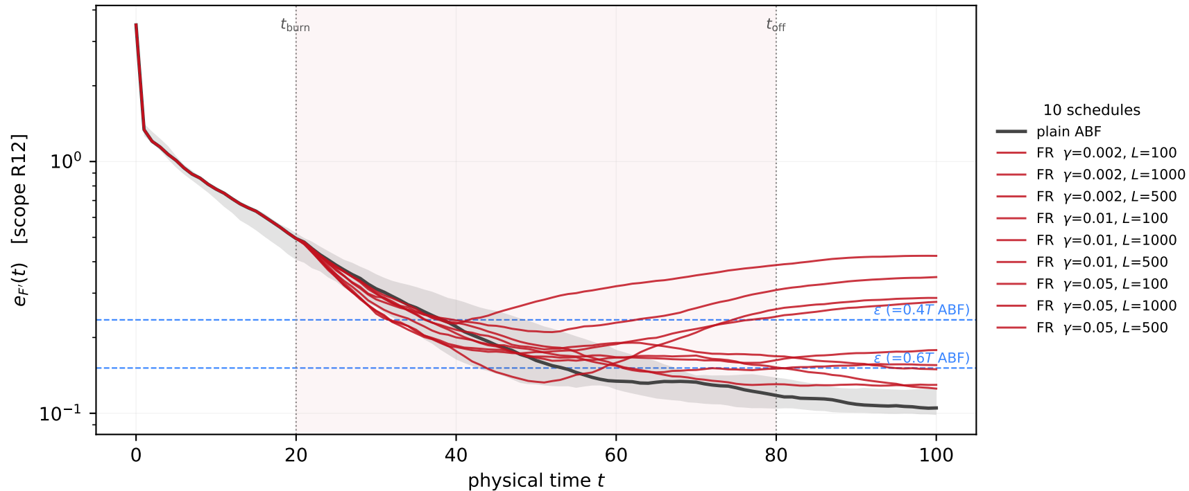
Mean-force convergence
