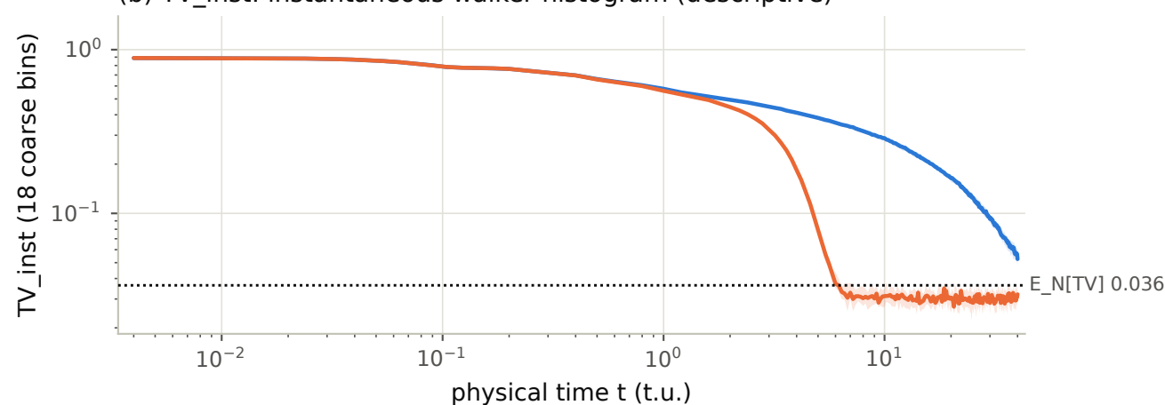
(b) TV_inst: instantaneous walker histogram (descriptive)
