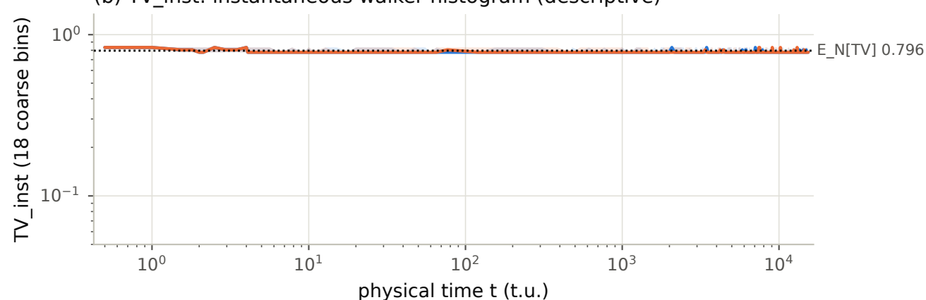
(b) TV_inst: instantaneous walker histogram (descriptive)
