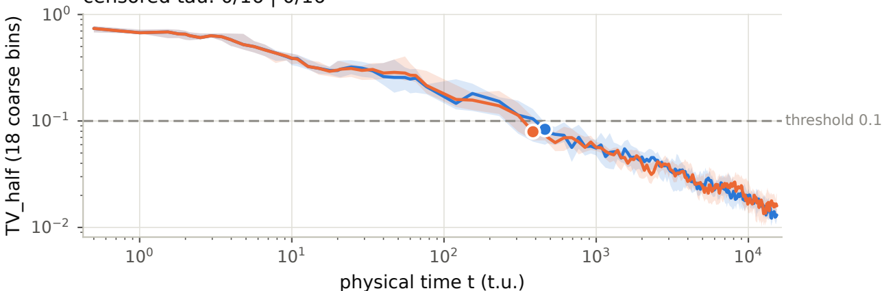
(a) TV_half: visitation over the trailing half C_{all}(t) - C_{all}(\approx t/2)
