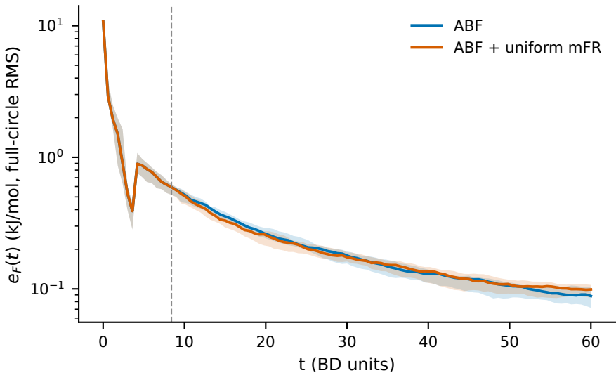
Ethane/LTA 300 K (16 paired seed labels, N=1024)
