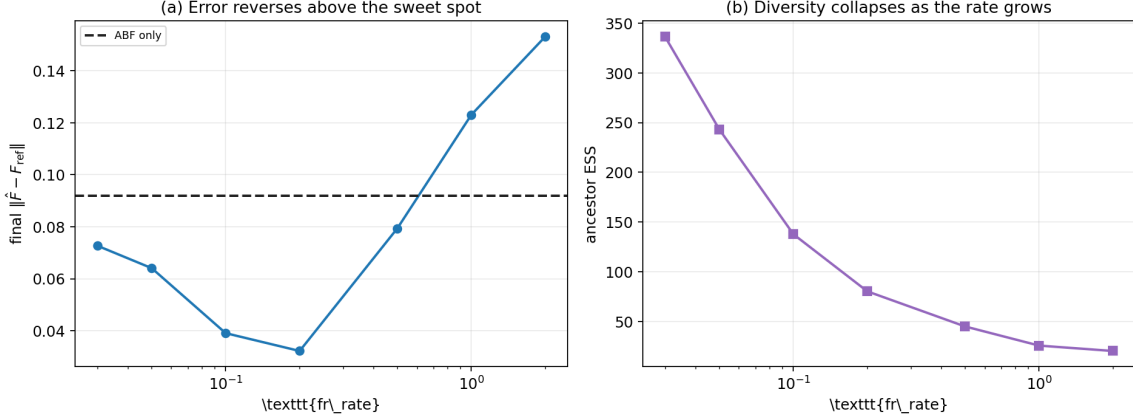
Figure 16: FR-rate ladder (150k steps, 4 seeds). Final L^2(F) (left) is minimised in the 0.1–0.2 sweet spot, climbs back toward the ABF baseline (dashed) by \text{fr\_rate}=0.5 , and rises above it for \text{fr\_rate} \geq 1 ; ancestor ESS (right) collapses as the rate grows, pinpointing diversity loss as the failure mechanism.
