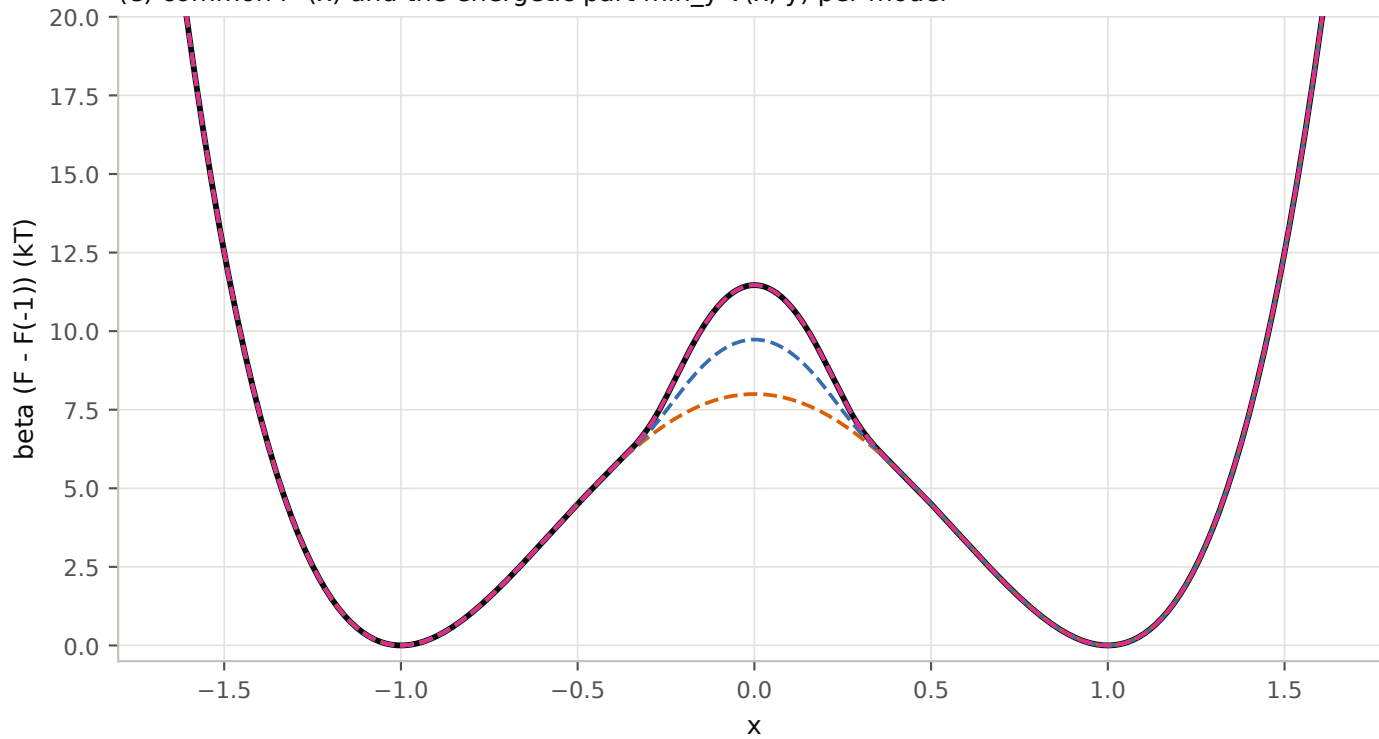
(e) common F^*(x) and the energetic part \min_y V(x, y) per model
