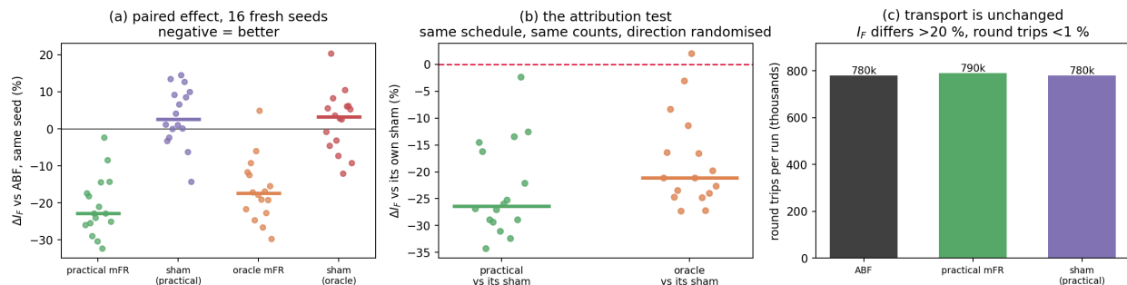
Figure 30: The matched-sham control on the WCA dimer, 16 fresh seeds at the accepted cell. (a) Paired per-seed change in the integrated free-energy error against ABF on the same seed; bars are medians. Both mFR arms sit below zero, both shams above it. (b) The attribution test: each arm against its own sham, which fired the same number of clone and delete events at the same times and differs only in which replicas it acted on. (c) Round trips per run differ by under 1% across arms while the free energy differs by more than twenty — the mechanism redistributes population rather than creating barrier crossings.
