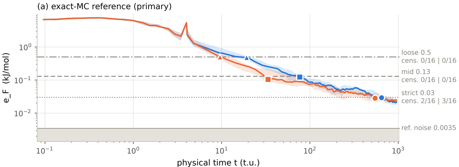
Free-energy error e_F vs physical time
