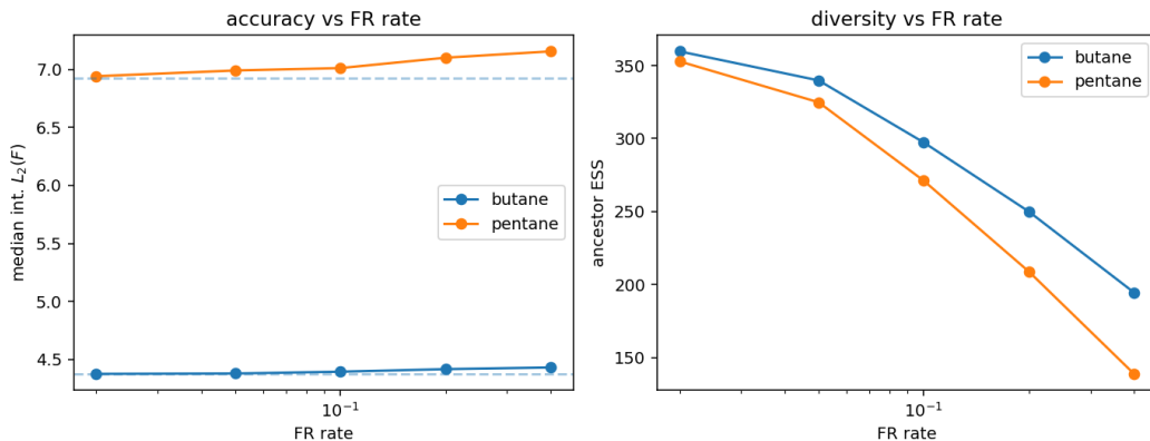
Figure 34: mFR rate ladder on the alkanes: accuracy (integrated L_2(F) ) and ancestor ESS versus FR rate, identifying the useful window (if any) and the over-aggressive boundary.
