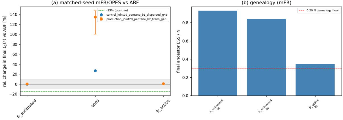
Figure 39: Matched-seed relative change in final L_2(F) of each method vs ABF (left; the shaded band is the \pm 10\% practical-equivalence margin, the dashed line the -15\% positive threshold) and the final ancestor ESS of each mFR configuration (right; the dashed line is the 0.30 N genealogy floor).
