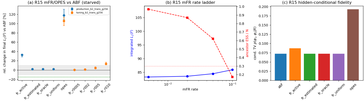
Figure 36: R_{15} mFR/OPES on the starved \beta = 2 cell: (a) matched-seed relative change in final L_2(F) vs ABF (band = \pm 10\% equivalence, dashed = -15\% positive threshold); (b) the mFR rate ladder — integrated L_2 rises and ancestor ESS collapses with rate, no useful window; (c) hidden-conditional p(\phi_1, \phi_2 | R) fidelity per method.
