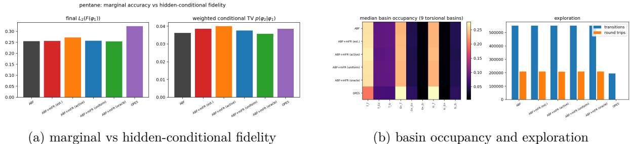
Figure 33: Pentane hidden-coordinate diagnostics: whether a method’s \varphi_1 accuracy is matched by faithful p(\varphi_2|\varphi_1) (left) and how it populates the nine torsional basins (right).
