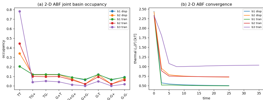
Figure 38: 2-D ABF starvation screen: joint nine-basin occupancy (left) and thermal-window L_2(F) convergence (right) across the P2 cells.
