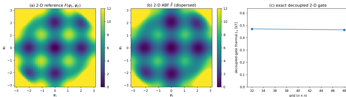
Figure 37: (a) the joint reference F(\varphi_1, \varphi_2) ; (b) a representative 2-D ABF reconstruction; (c) the exact decoupled gate L_2 versus grid resolution — flat, showing the residual is the mean-force estimator floor rather than a grid-discretisation error.
