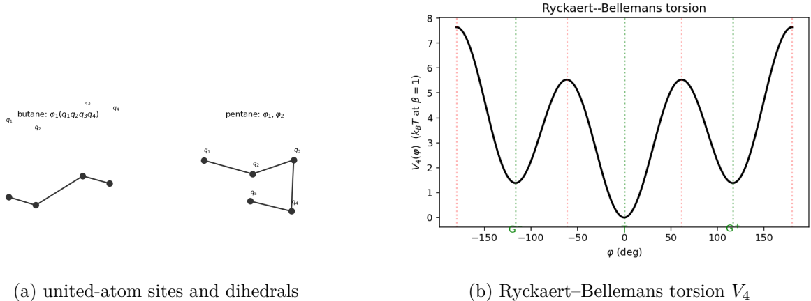
Figure 30: Molecular models and the torsional potential. Trans is \varphi = 0 ( V_4 = 0 ), gauche \pm 116.6^\circ ( 1.38 k_B T ), trans-gauche barrier 5.53 k_B T , cis barrier 7.64 k_B T .
