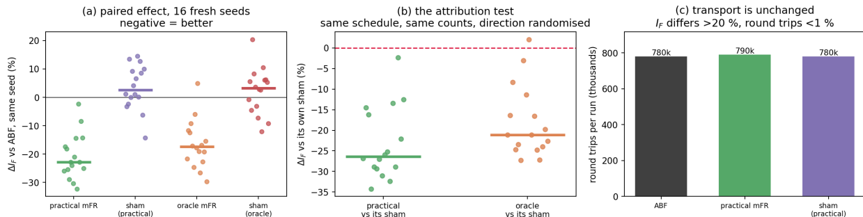
Figure 29: The matched-sham control on the WCA dimer, 16 fresh seeds at the accepted cell. (a) Paired per-seed change in the integrated free-energy error against ABF on the same seed; bars are medians. Both mFR arms sit below zero, both shams above it. (b) The attribution test: each arm against its own sham, which fired the same number of clone and delete events at the same times and differs only in which replicas it acted on. (c) Round trips per run differ by under 1% across arms while the free energy differs by more than twenty — the mechanism redistributes population rather than creating barrier crossings.
