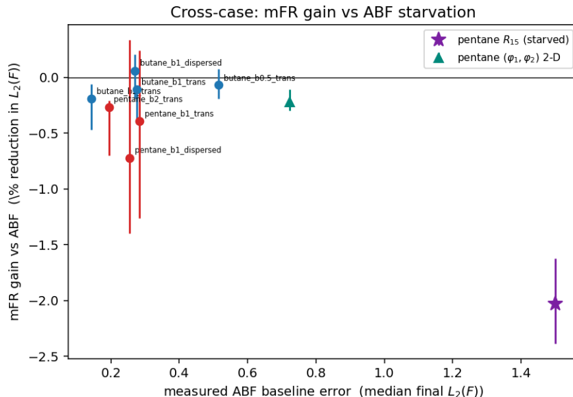
Figure 40: Cross-case starvation map: matched-seed mFR gain versus measured ABF baseline error, with the butane and pentane \varphi_1 points overlaid on the WCA regime cells (grey). The collective-variable extension adds the two decisive points: the pentane R_{15} cell (purple star) sits at the largest measured ABF error anywhere in the study yet returns a negative mFR gain, and the 2-D torsion cell (teal triangle) is likewise flat. The WCA-derived reading — that measured ABF error predicts mFR gain — therefore does not extrapolate to molecular coordinates: high ABF error is necessary but not sufficient, because R_{15} starvation is dynamical (rare barrier crossing) rather than a marginal support deficit that reallocation can repair.
