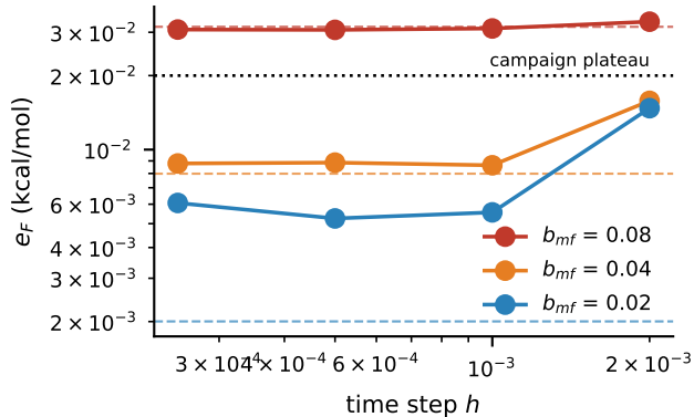
butane, warm constrained TI (dashed = analytic smoothing floor)
