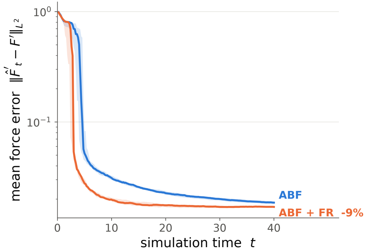
Mean force
