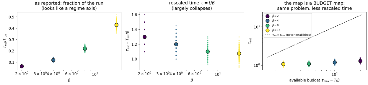
Figure 41: The \beta axis collapses under the rescaling of Equation (36). Left: as originally reported, the establishment time as a fraction of the run varies 6.62\times across the ladder, which reads like a regime axis. Middle: in rescaled time \tau = t/\beta it varies 1.21\times against an 8\times change in \beta , and \tau_{\text{hit}} is identical to four digits. Right: the same points against the available budget \tau_{\text{max}} = T/\beta , which is what the ladder actually varies. Small points are individual runs, large points the median over the 16 seeds and 16 (s, r) cells at that \beta . The residual drift is downward in \beta , the sign predicted by finite- \beta non-adiabaticity of the transverse channel.
