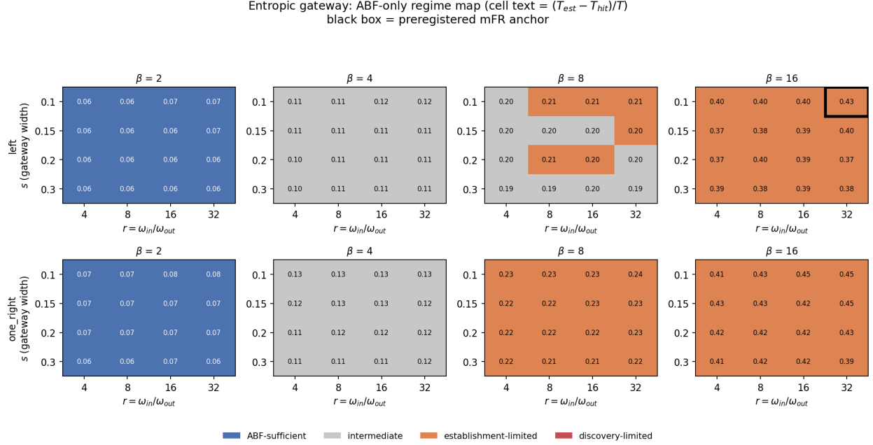
Figure 42: ABF-only regime map of the entropic gateway, all 128 cells. Rows are the two initialisations, columns the transport ladder \beta ; each panel is the (s, r) plane and each tile is annotated with the establishment gap (T_{\text{est}} - T_{\text{hit}})/T . The dimensionless landscape is identical in every tile ( \beta H = 8 k_B T fixed), so the layering in \beta is a statement about timescales, not about thermodynamics. The black box marks the preregistered mFR anchor. Within a fixed \beta the gateway geometry modulates the gap only at the margin — a result, not a nuisance, and the reason the whole map is shown rather than one slice.
