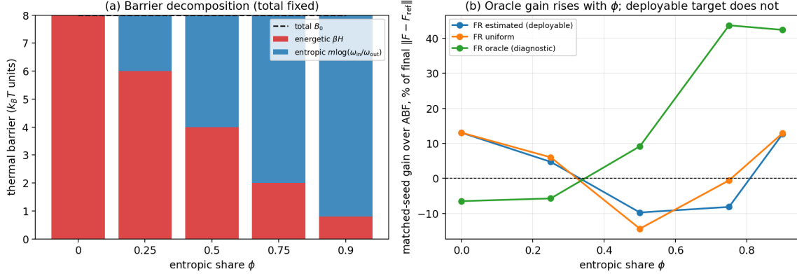
Figure 13: Entropy-dominant stress test at fixed total barrier B_0 . (a) The barrier decomposition: as \phi grows the energetic part \beta H is traded for the entropic part m \log(\omega_{\text{in}}/\omega_{\text{out}}) with the total held constant. (b) Matched-seed gain over ABF: the deployable estimated (and uniform) targets are small and non-monotone in \phi , whereas the oracle gain rises sharply with the entropic share — the achievable benefit is entropic-specific, but the practical online estimate does not capture it.
