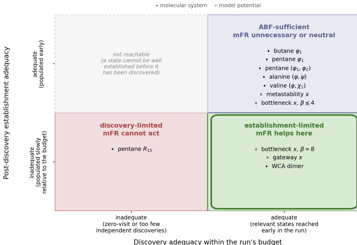
Figure 46: The regime map, on categorical axes. Both axes are two-state because that is what the evidence supports: each system carries a discovery verdict and an establishment verdict, not a continuous adequacy score, and interpolating coordinates to draw a scatter plot would present a classification as a measurement. The upper-left cell is empty by construction — a state cannot be well established before it has been discovered. Only the outlined cell is mFR’s. Generated from results/closure/v1_regime_map.csv by report/scripts/make_regime_map_figure.py .
