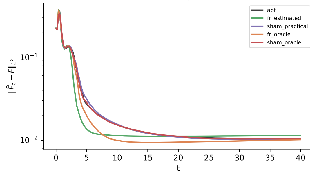
free-energy error
