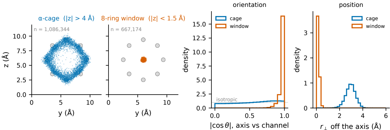
Ethane in LTA, 150 K: COM cross-section (y, z) and orientation in the cage vs in the window (abf arm, t \in [4, 60] )
