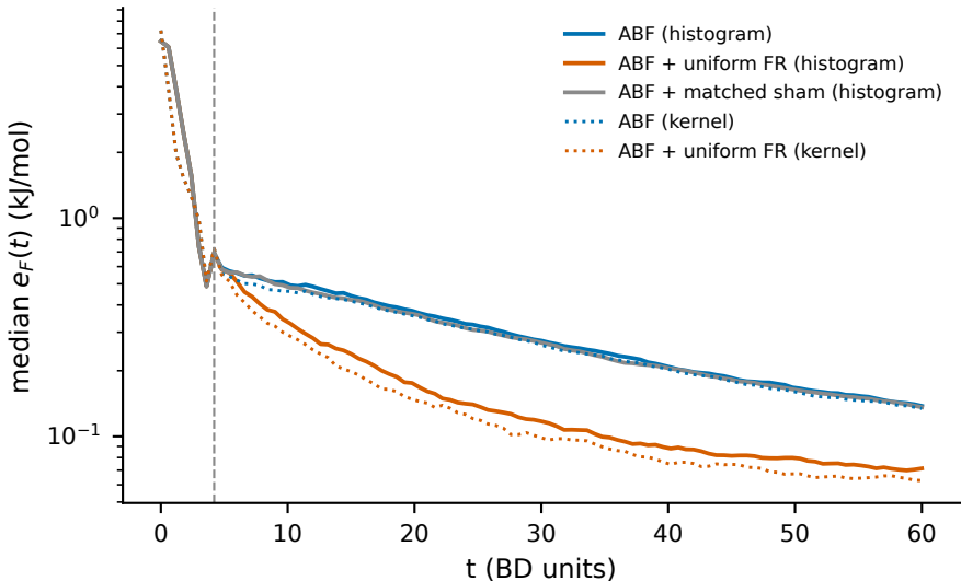
Ethane/LTA 150 K: histogram (solid) vs kernel (dotted), 16 seeds
