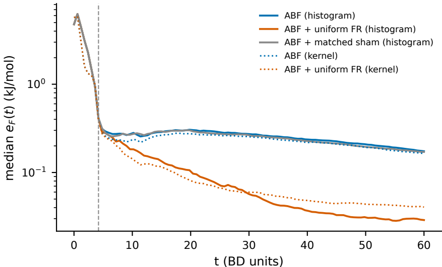
Ethane/LTA 80 K: histogram (solid) vs kernel (dotted), 16 seeds
