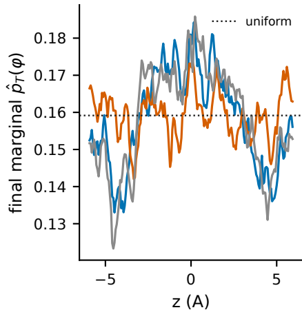
Ethane/LTA 150 K, histogram estimator: final median profiles (window at z=0 , cages at \pm a/2 )
