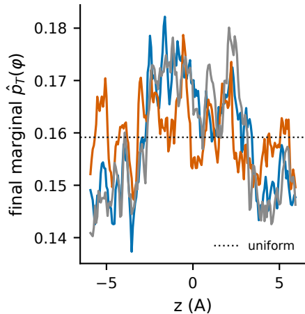
Ethane/LTA 225 K, histogram estimator: final median profiles (window at z=0 , cages at \pm a/2 )
