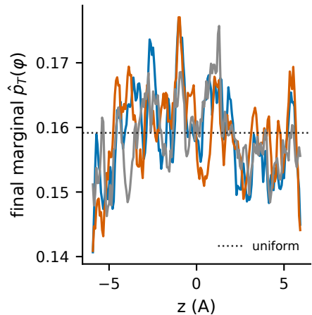
Ethane/LTA 300 K, histogram estimator: final median profiles (window at z=0 , cages at \pm a/2 )
