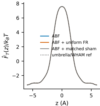
Ethane/LTA 300 K, histogram estimator: final median profiles (window at z=0 , cages at \pm a/2 )
