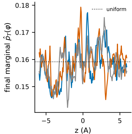
Ethane/LTA 350 K, histogram estimator: final median profiles (window at z=0 , cages at \pm a/2 )
