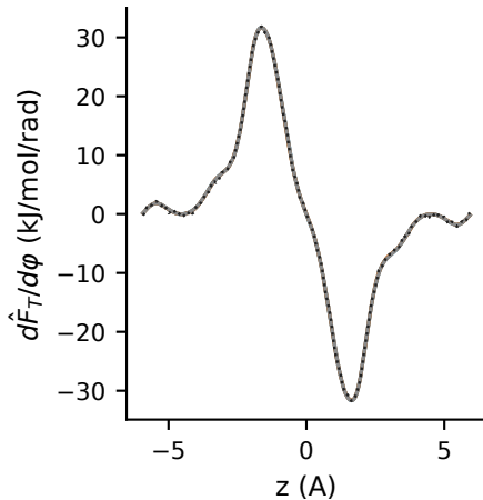
Ethane/LTA 350 K, histogram estimator: final median profiles (window at z=0 , cages at \pm a/2 )
