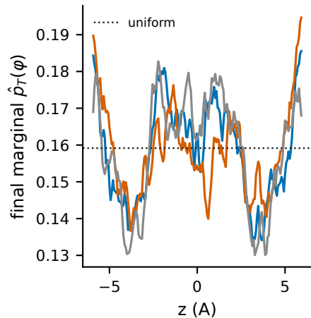
Ethane/LTA 80 K, histogram estimator: final median profiles (window at z=0 , cages at \pm a/2 )
