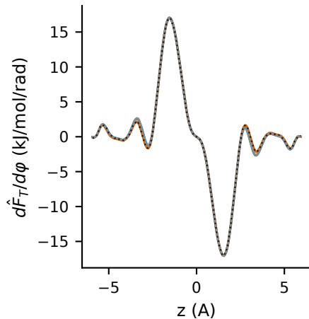
Ethane/LTA 80 K, histogram estimator: final median profiles (window at z=0 , cages at \pm a/2 )
