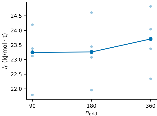
Ethane/LTA 300 K width ladder (ABF only, histogram estimator, R=4 noise-paired seeds)
