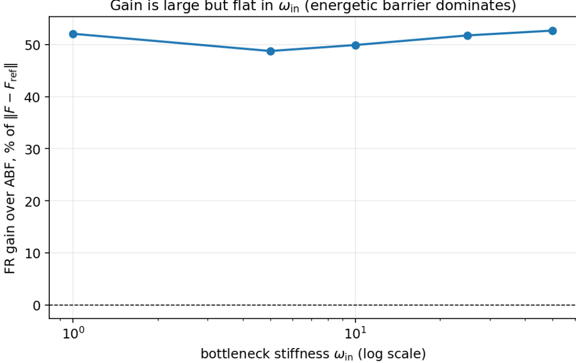
Figure 10: Bottleneck-width sweep \omega_{\text{in}} at \beta = 8 . The FR gain is large ( \sim 50\% ) and 100% reliable at every width, but it does not grow with the bottleneck strength: the ABF baseline error is flat because the energetic barrier height H = 2.5 dominates the smaller entropic contribution \beta^{-1} \log(\omega_{\text{in}}/\omega_{\text{out}}) .
