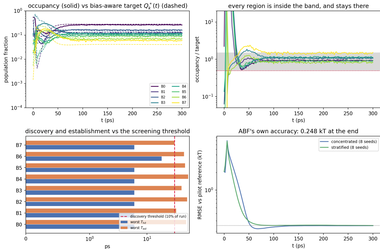
Figure 42: Ace-Val-Nme, the decisive gate. Top left: region occupancy (solid) against the bias-aware target Q_k^*(t) of Equation (34) (dashed), all eight regions over three decades of population. Top right: the same as a ratio; every region enters the establishment band and stays there. Bottom left: worst-case hitting and establishment times against the discovery threshold. Bottom right: ABF's own accuracy, with the concentrated and stratified initialisations giving the same answer — the diagnostic control doing its job, since the verdict is then not an artifact of where the walkers started.
