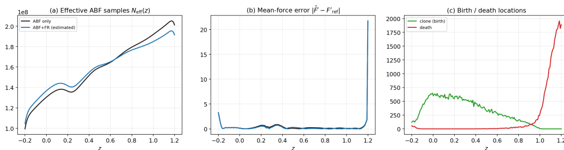
Figure 16: Mechanism. (a) The kernel-weighted ABF denominator N_{\text{eff}}(z) is raised by FR in the transition window; (b) per-bin mean-force error is reduced there; (c) birth (clone) and death locations concentrate around the over/under-sampled regions; FR reshapes the sampling support , not the stationary marginal.
