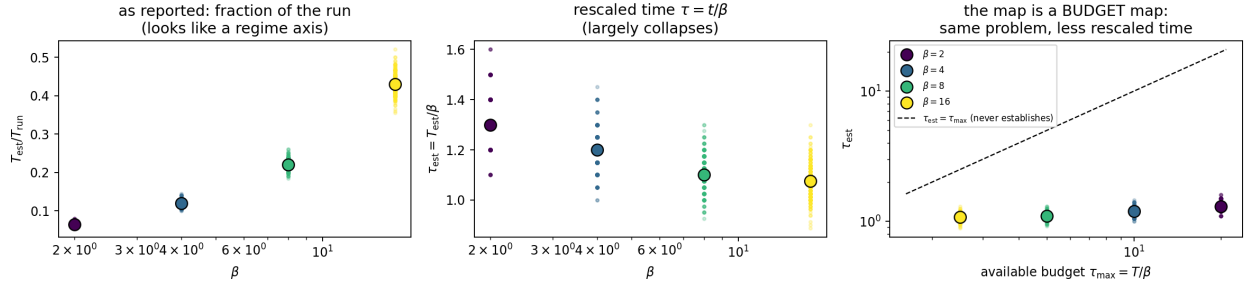
Figure 43: The \beta axis collapses under the rescaling of Equation (36). Left: as originally reported, the establishment time as a fraction of the run varies 6.62\times across the ladder, which reads like a regime axis. Middle: in rescaled time \tau = t/\beta it varies 1.21\times against an 8\times change in \beta , and \tau_{\text{hit}} is identical to four digits. Right: the same points against the available budget \tau_{\text{max}} = T/\beta , which is what the ladder actually varies. Small points are individual runs, large points the median over the 16 seeds and 16 (s, r) cells at that \beta . The residual drift is downward in \beta , the sign predicted by finite- \beta non-adiabaticity of the transverse channel.
