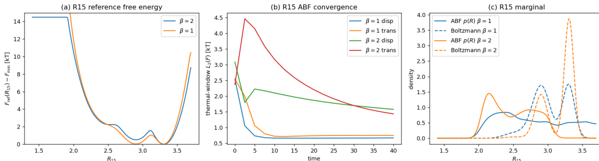
Figure 34: Pentane R_{15} : (a) reference free energy (minimum at the extended state, compact configurations strongly disfavoured); (b) ABF convergence of the thermal-window L_2(F) for the four screen cells — the \beta=2 cells remain far above the \beta=1 ones (1.43–1.58 vs 0.67–0.74 kT); (c) the ABF-sampled R_{15} marginal (solid) against the unbiased Boltzmann law (dashed, same colour): ABF broadens the marginal towards compact R as intended, but the residual structure at \beta=2 is the support deficit the screen detects.
