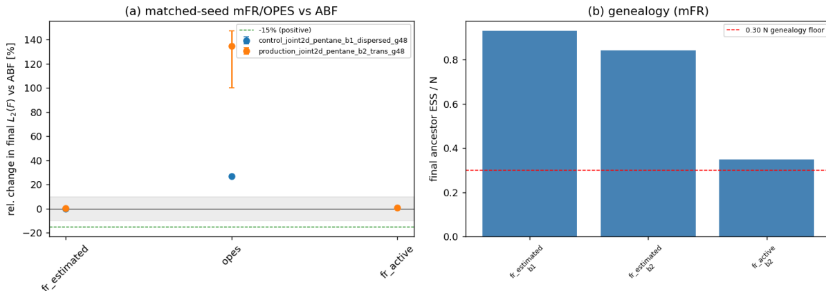
Figure 38: Matched-seed relative change in final L_2(F) of each method vs ABF (left; the shaded band is the \pm 10\% practical-equivalence margin, the dashed line the -15\% positive threshold) and the final ancestor ESS of each mFR configuration (right; the dashed line is the 0.30 N genealogy floor).
