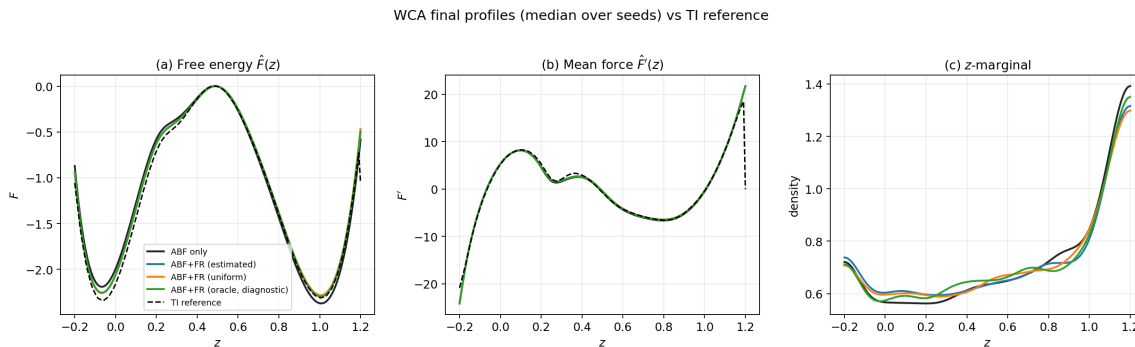
Figure 14: Final profiles (median over seeds) versus the TI reference (dashed): (a) free energy \hat{F}(z) , (b) mean force \hat{F}'(z) , (c) reaction-coordinate marginal. FR recovers the reference free energy more accurately than ABF, chiefly in and around the transition region.
