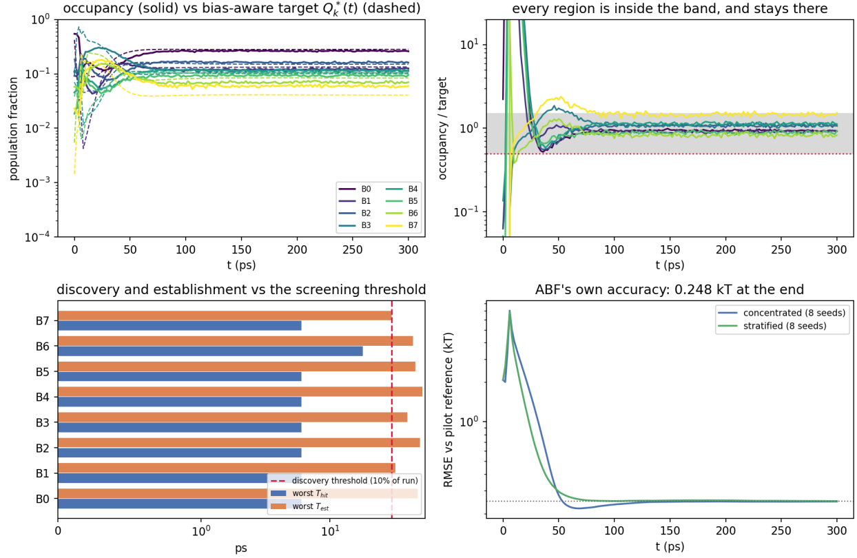
Figure 40: Ace-Val-Nme, the decisive gate. Top left: region occupancy (solid) against the bias-aware target Q_k^*(t) of Equation (34) (dashed), all eight regions over three decades of population. Top right: the same as a ratio; every region enters the establishment band and stays there. Bottom left: worst-case hitting and establishment times against the discovery threshold. Bottom right: ABF's own accuracy, with the concentrated and stratified initialisations giving the same answer — the diagnostic control doing its job, since the verdict is then not an artifact of where the walkers started.
