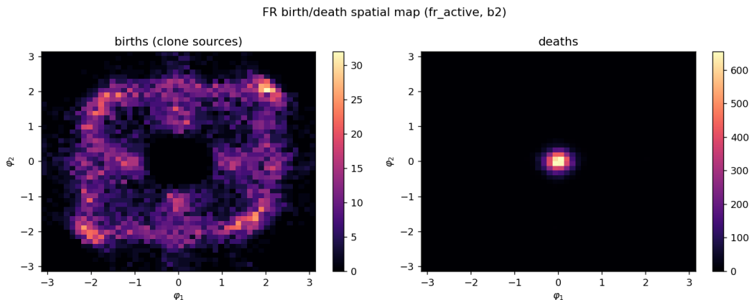
Figure 39: Spatial birth (clone-source) and death maps of the 2-D mFR birth-death process on the torsion torus, showing where reallocation moves probability mass.
