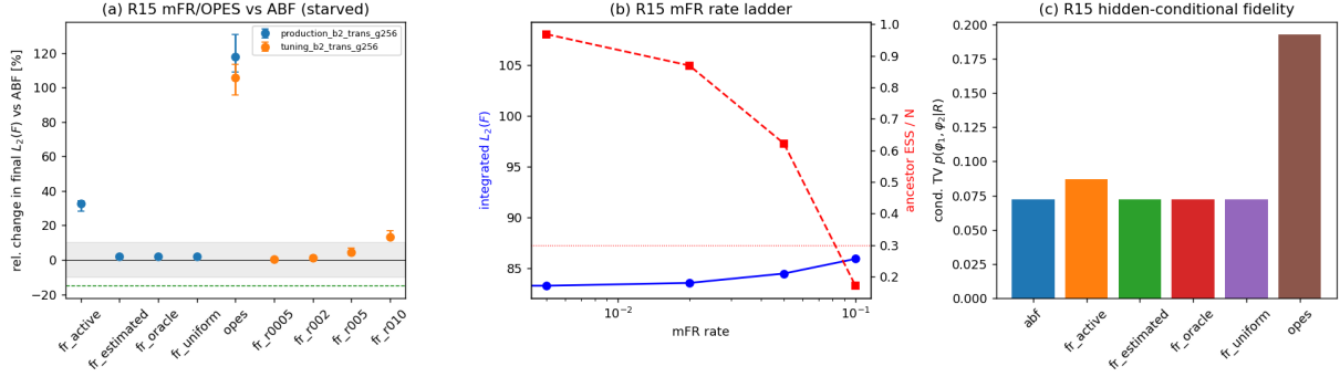
Figure 35: R_{15} mFR/OPES on the starved \beta = 2 cell: (a) matched-seed relative change in final L_2(F) vs ABF (band = \pm 10\% equivalence, dashed = -15\% positive threshold); (b) the mFR rate ladder — integrated L_2 rises and ancestor ESS collapses with rate, no useful window; (c) hidden-conditional p(\varphi_1, \varphi_2 | R) fidelity per method.
