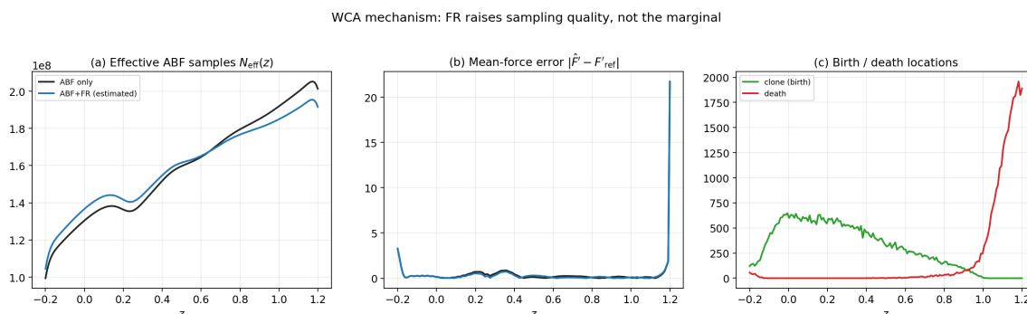
Figure 15: Mechanism. (a) The kernel-weighted ABF denominator N_{\text{eff}}(z) is raised by FR in the transition window; (b) per-bin mean-force error is reduced there; (c) birth (clone) and death locations concentrate around the over/under-sampled regions; FR reshapes the sampling support , not the stationary marginal.
