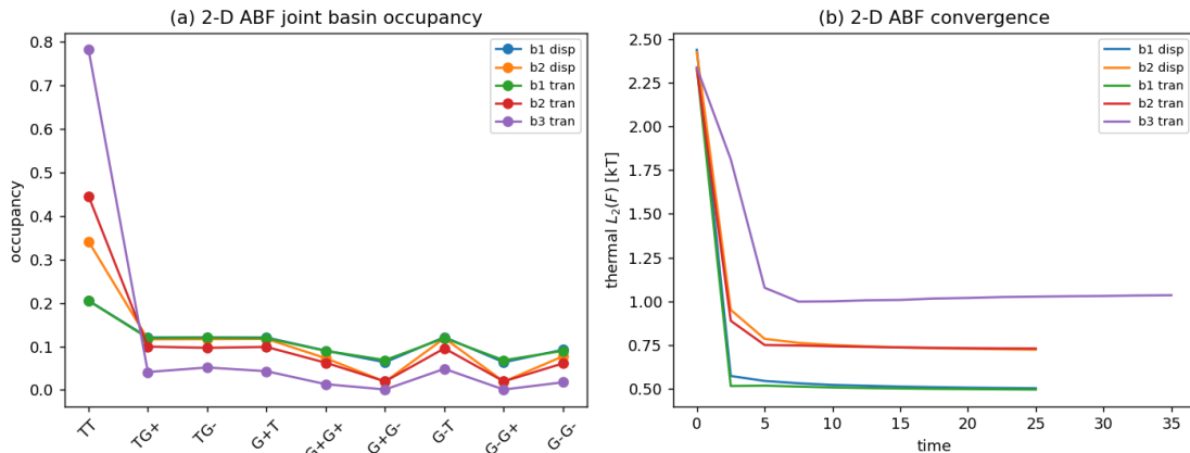
Figure 37: 2-D ABF starvation screen: joint nine-basin occupancy (left) and thermal-window L_2(F) convergence (right) across the P2 cells.
