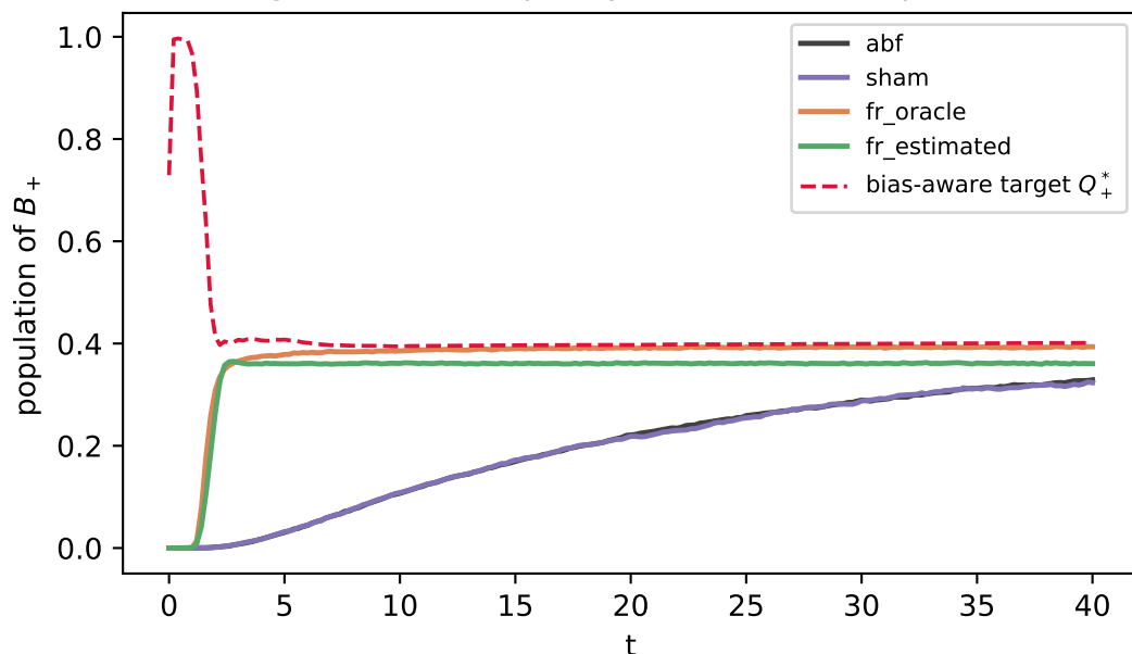
right-basin occupancy at the anchor ( \gamma = 15 )
