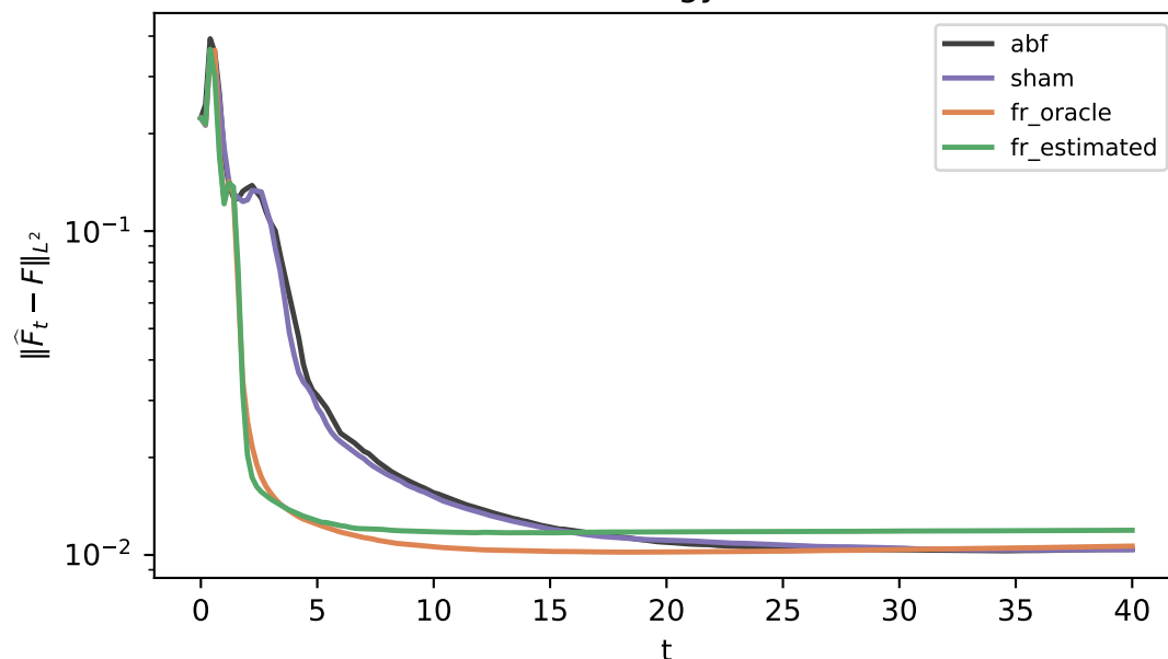
free-energy error
