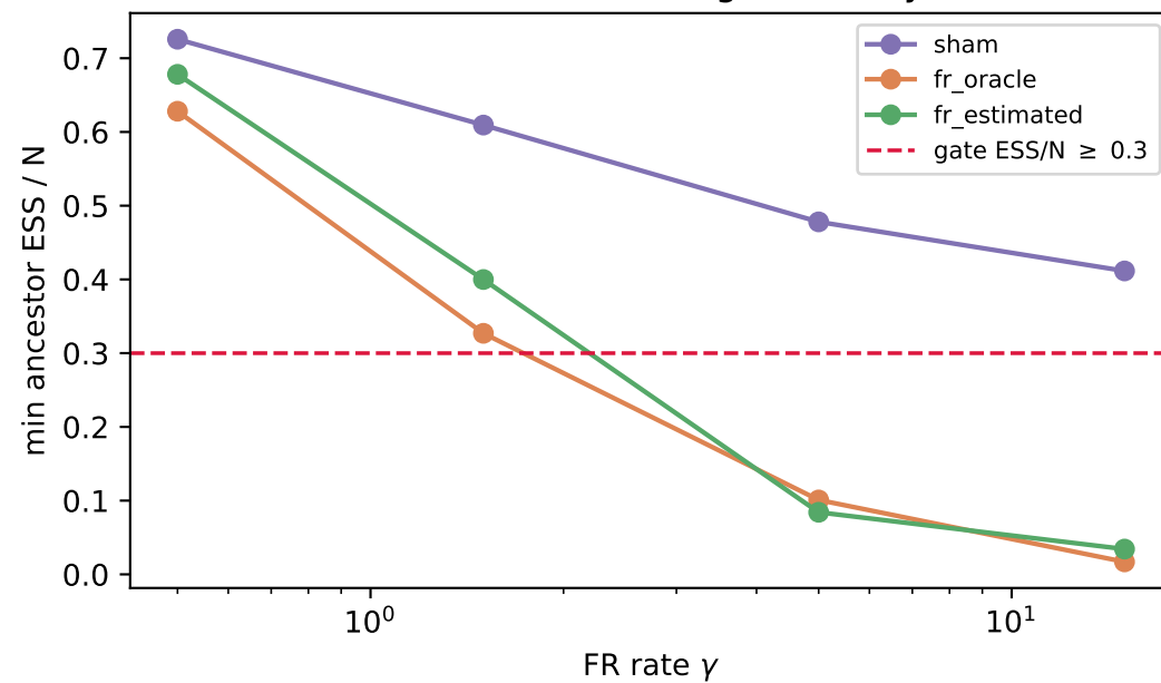
the cost side: lineage diversity
