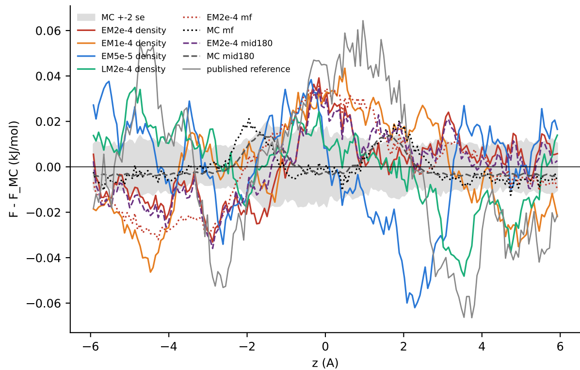
(b) differences from exact Gibbs
