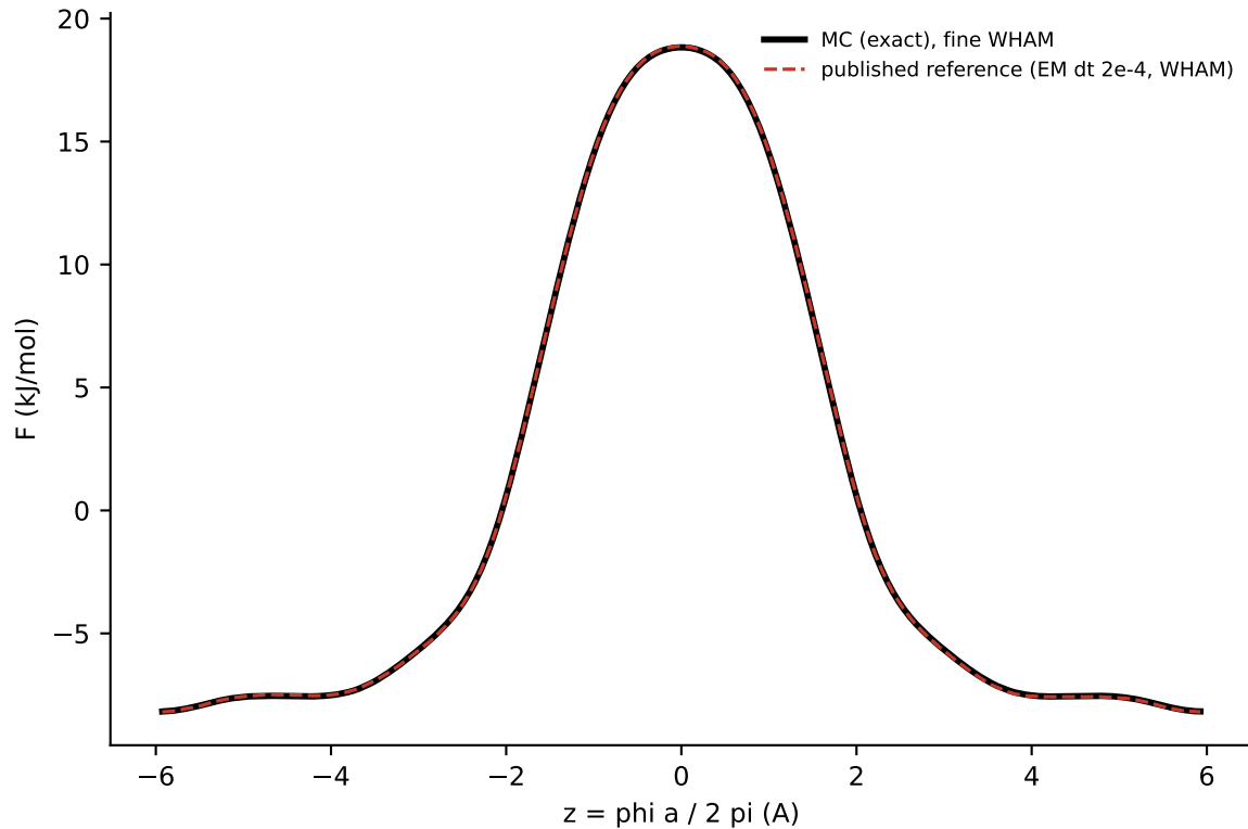
(a) ethane/LTA 300 K
