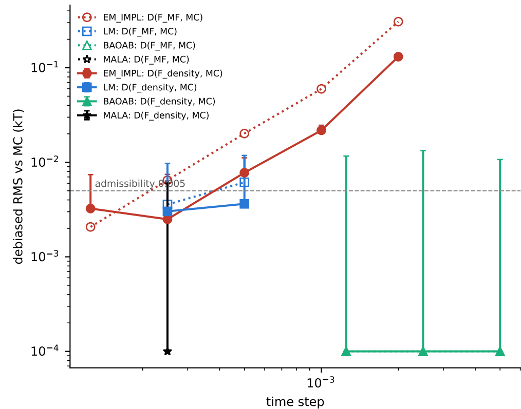
(c) timestep convergence
