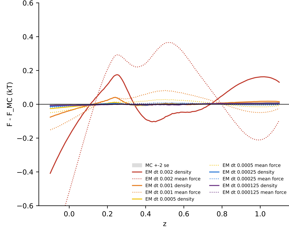
(b) production EM minus exact Gibbs
