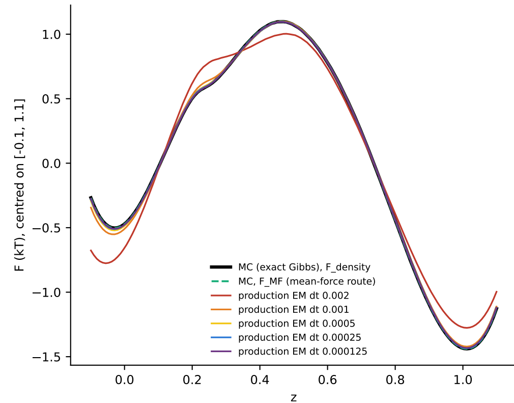
(a) free energy, density route
