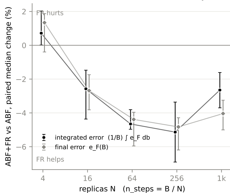
(b) Fisher-Rao benefit vs number of replicas
