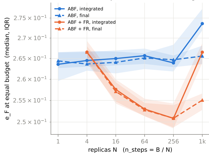
(c) which (N, T) split is best at fixed budget
