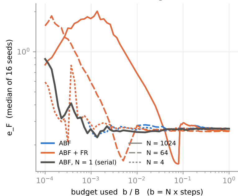
(a) error vs normalised budget
