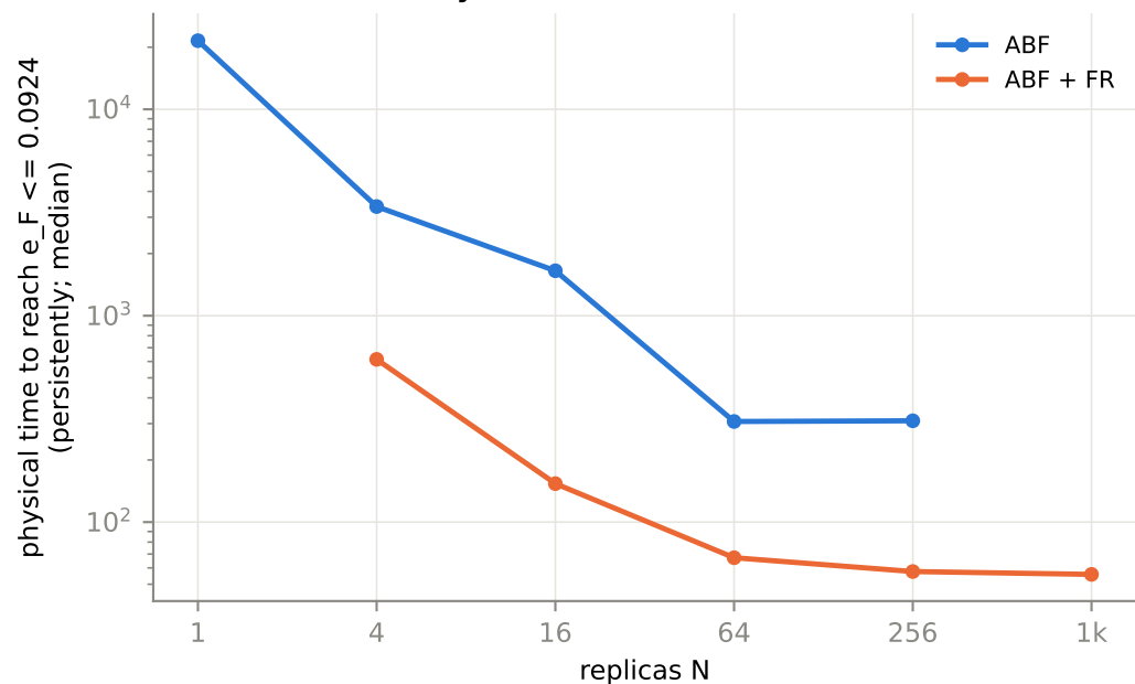
(b) time-to-accuracy
