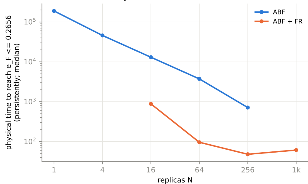
(b) time-to-accuracy
