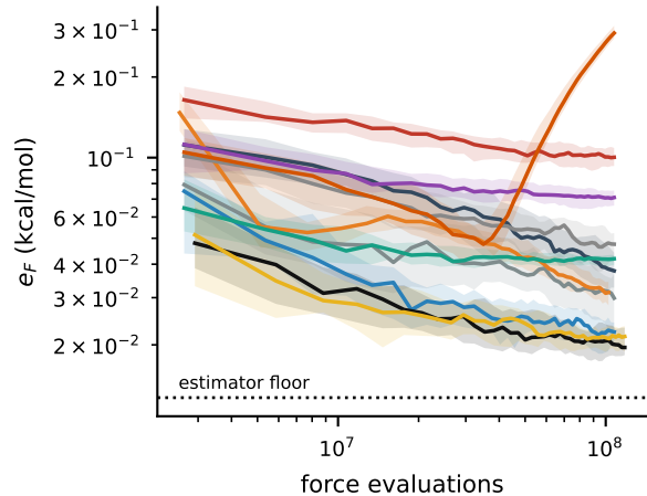
free-energy error
