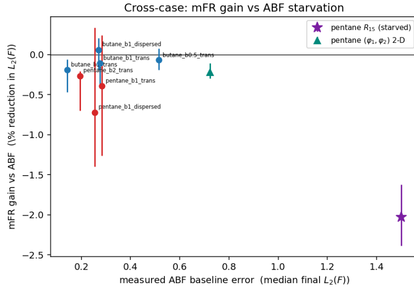
Figure 48: Cross-case starvation map: matched-seed mFR gain versus measured ABF baseline error, with the butane and pentane \varphi_1 points overlaid on the WCA regime cells (grey). The collective-variable extension adds the two decisive points: the pentane R_{15} cell (purple star) sits at the largest measured ABF error anywhere in the study yet returns a negative mFR gain, and the 2-D torsion cell (teal triangle) is likewise flat. The WCA-derived reading — that measured ABF error predicts mFR gain — therefore does not extrapolate to molecular coordinates: high ABF error is necessary but not sufficient, because R_{15} starvation is dynamical (rare barrier crossing) rather than a marginal support deficit that reallocation can repair.
